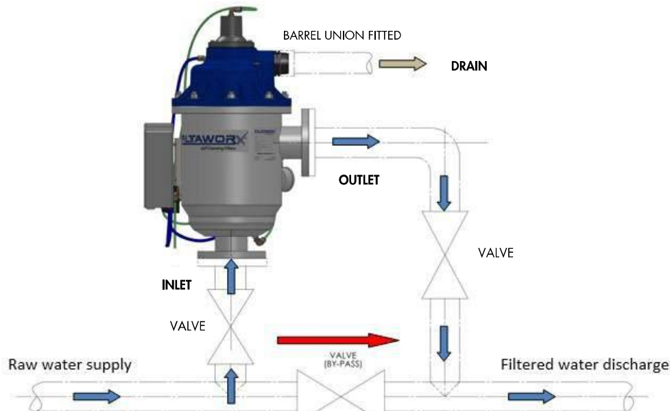
Figure 6 Filter Installation
